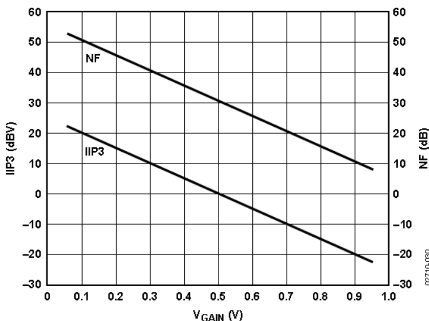
Figure 6. Noise Figure and Input Third-Order Intercept vs. Gain Voltage ( R_{\text{SOURCE}} = 200 \Omega )
