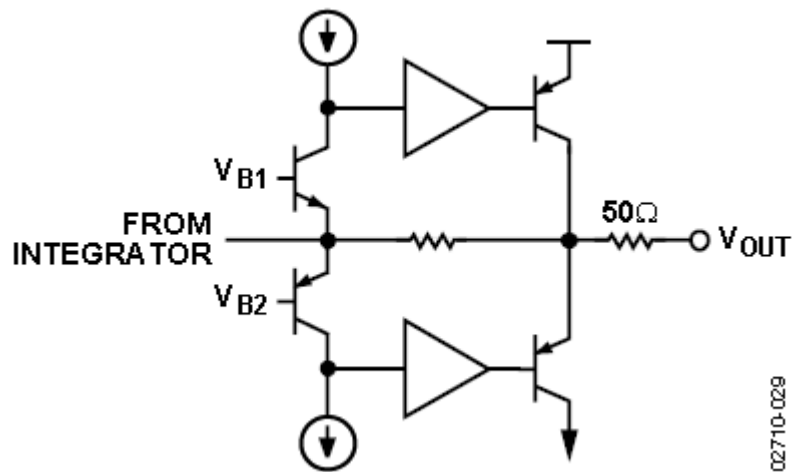
Figure 5. A 50 \Omega resistor is added to the output to prevent package resonance.
