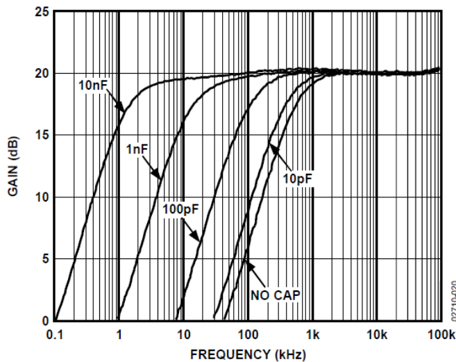
Figure 9. Gain vs. Frequency for Multiple Values of HPFL Capacitor a_g V_{GAIN} = 500\text{mV} .
