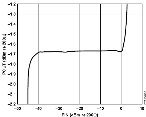
Figure 11: Leveling Accuracy of the AGC function.
