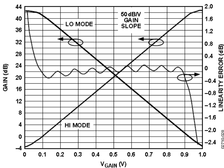
Figure 4. The gain function can be either an increasing or decreasing function of V_{GAIN} , depending on the MODE pin.
