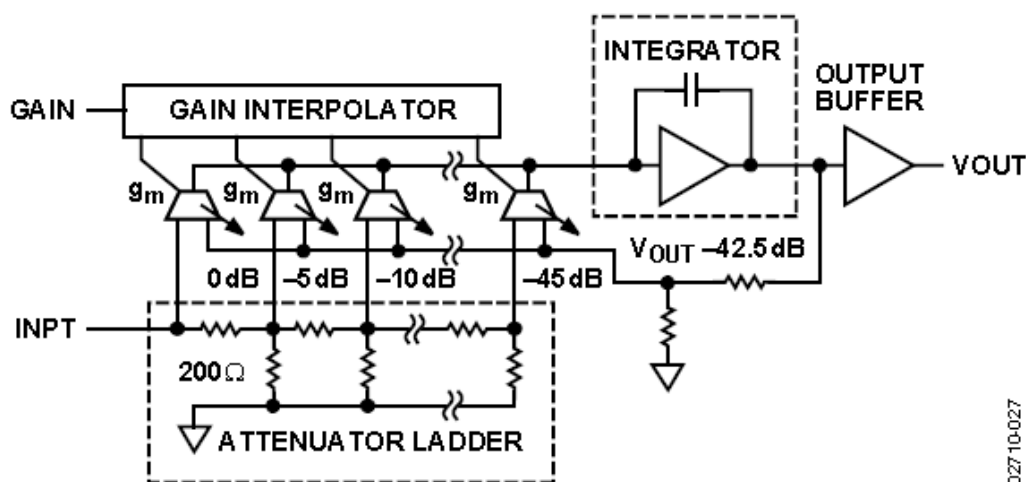
Figure 3 Simplified Architecture
